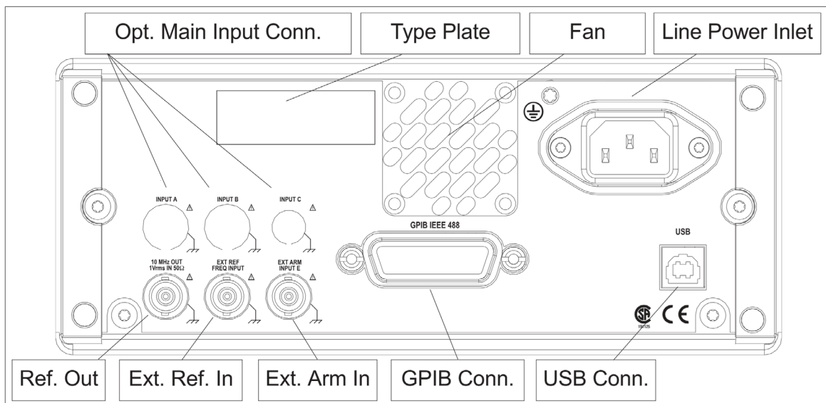
The CNT-90 rear panel layout.
