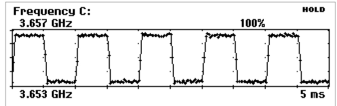
Figure 2: Pulse modulated frequency or FSK
