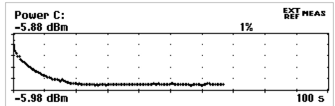
Figure 3: Generator start-up power settling
