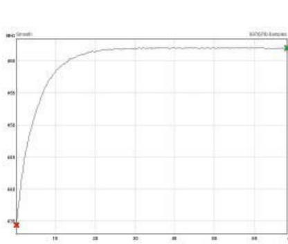
Figure 9: Frequency settling of VCO after step change of input voltage.
