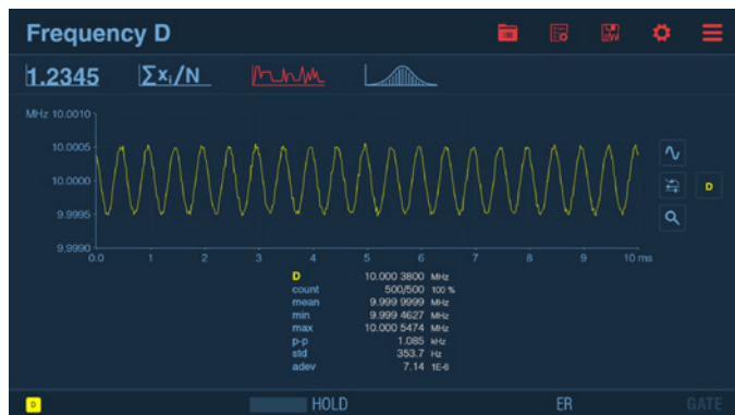
View fast FM, or any time/phase/frequency modulation, on screen, on one or more channels
